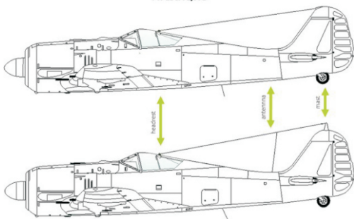
Fw 190A-4
